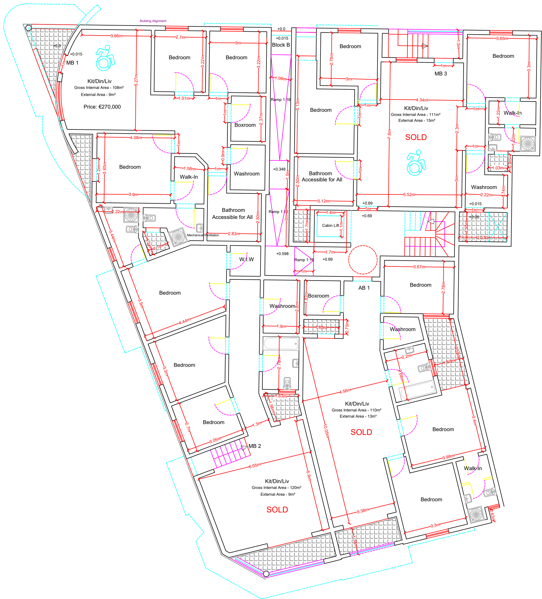
Approved/ Proposed Level 0 Scale 1:100
